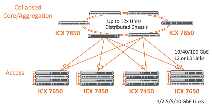
Figure 4: Two-tier campus network.
